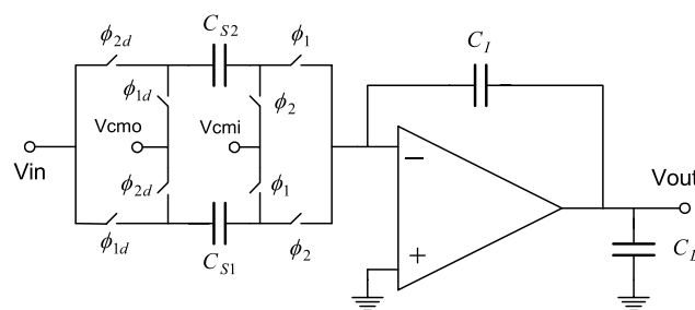
Fig. 1. A single-ended double-sampling integrator.
