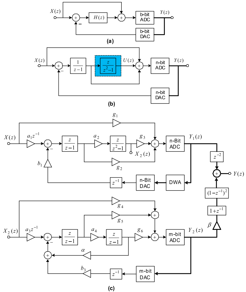
Fig. 2. General structure of a sigma-delta modulator, (b) the proposed second-order double-sampling modulator, and (c) the proposed double-sampling cascade 2-2 modulator topology.
