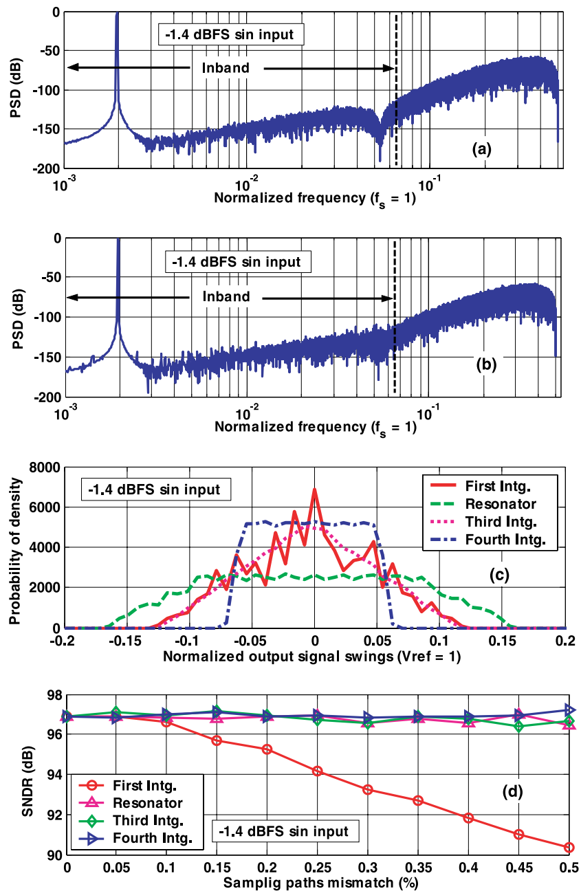
Fig. 3. Simulated ideal output spectrum, (b) output spectrum including the circuit non-idealities, (c) building blocks output swings, and (d) SNDR degradation versus the sampling paths mismatch.
