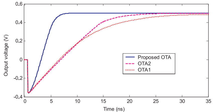
Fig. 2. Settling simulation results.
